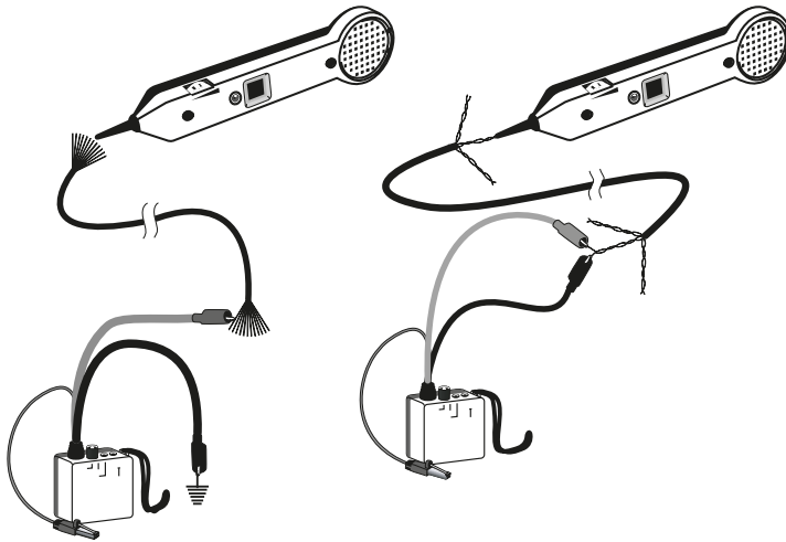
Figure 4a. Cable Tracing
